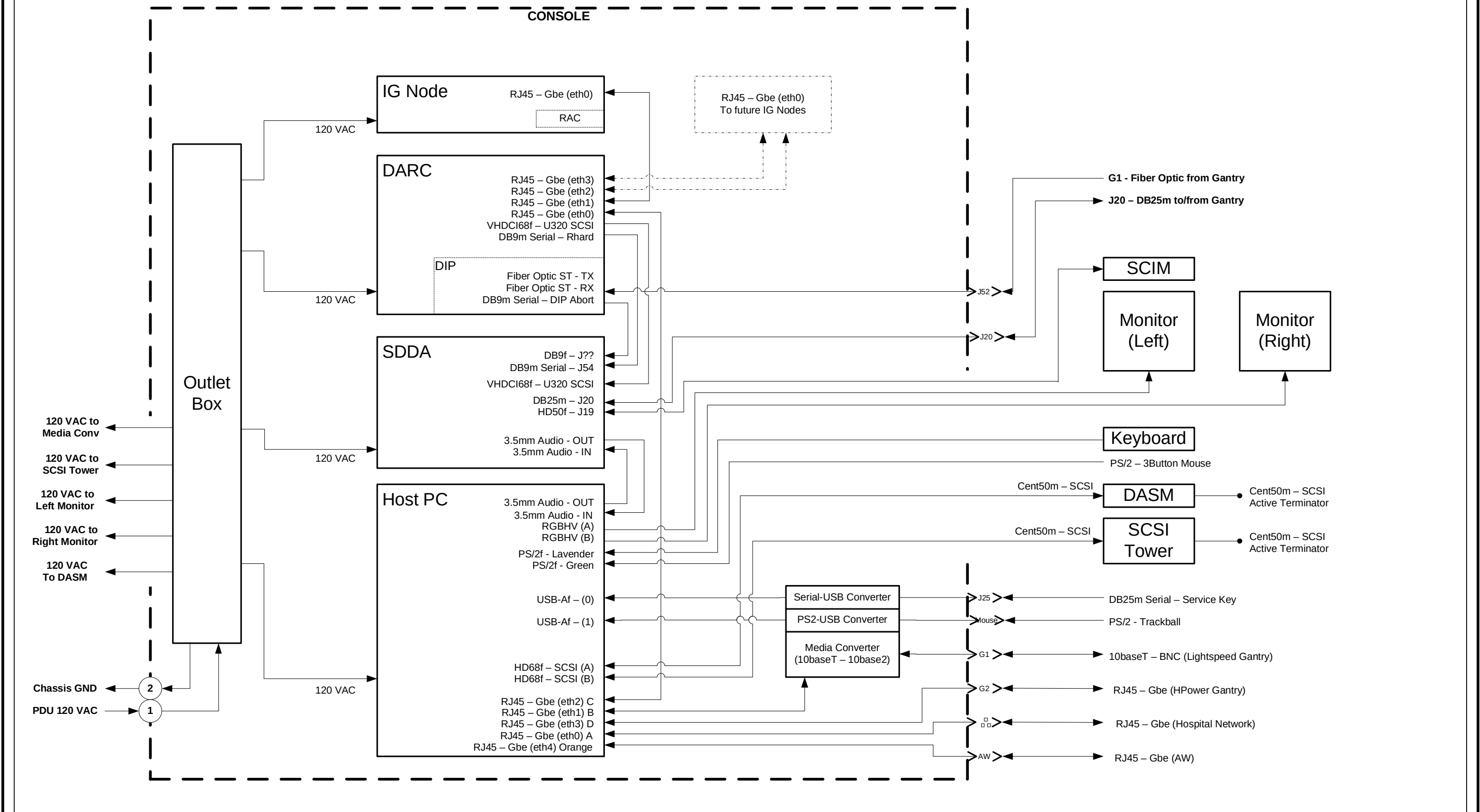
HP_Console Block Diagram
